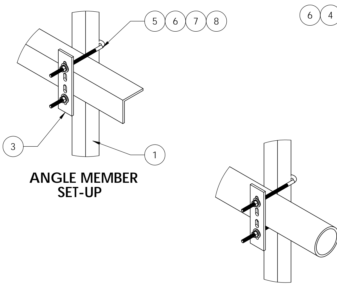
ROUND MEMBER SET-UP
